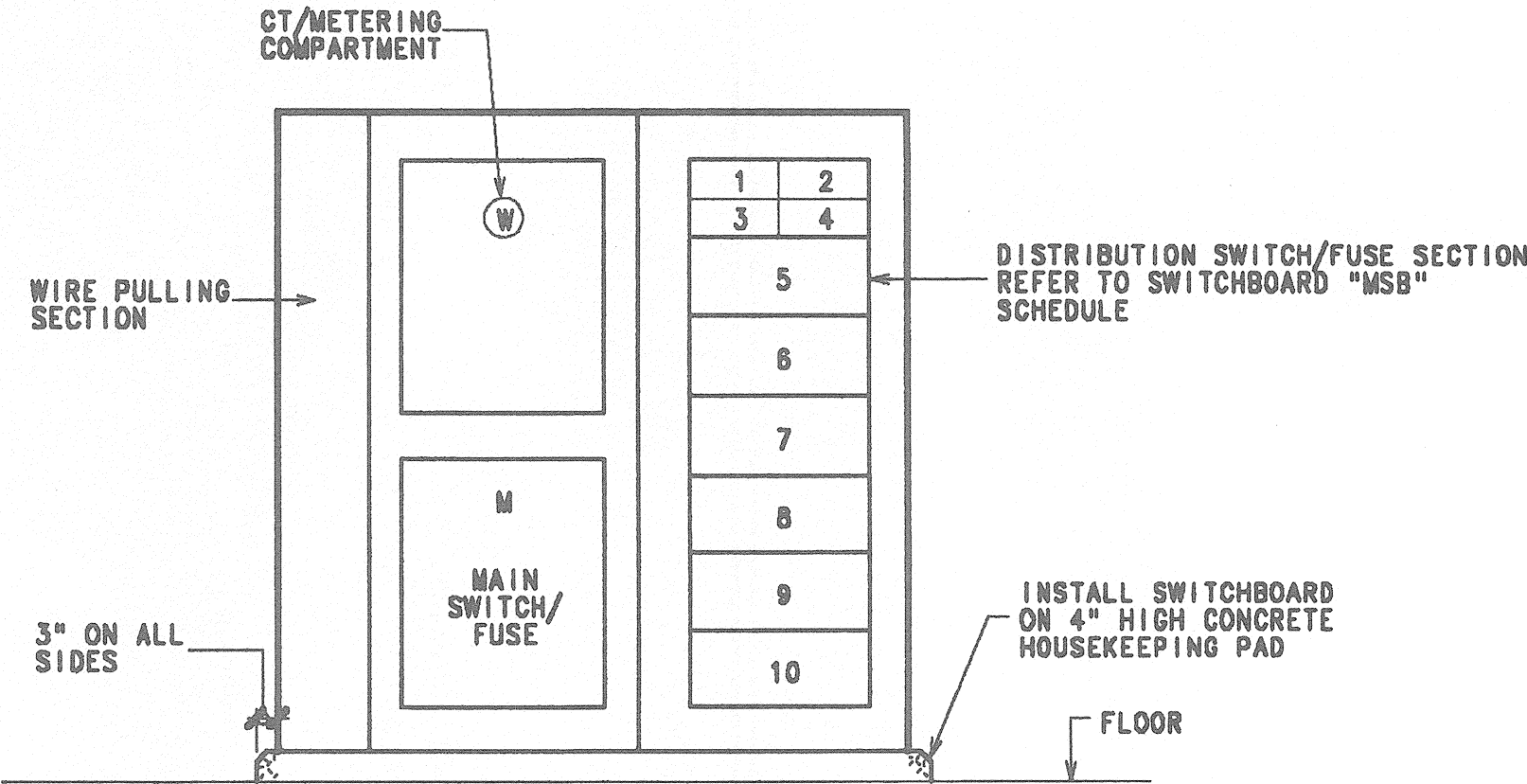
ELEVATION - SWITCHBOARD "MSB" SCALE: 1/2" = 1'-0"
