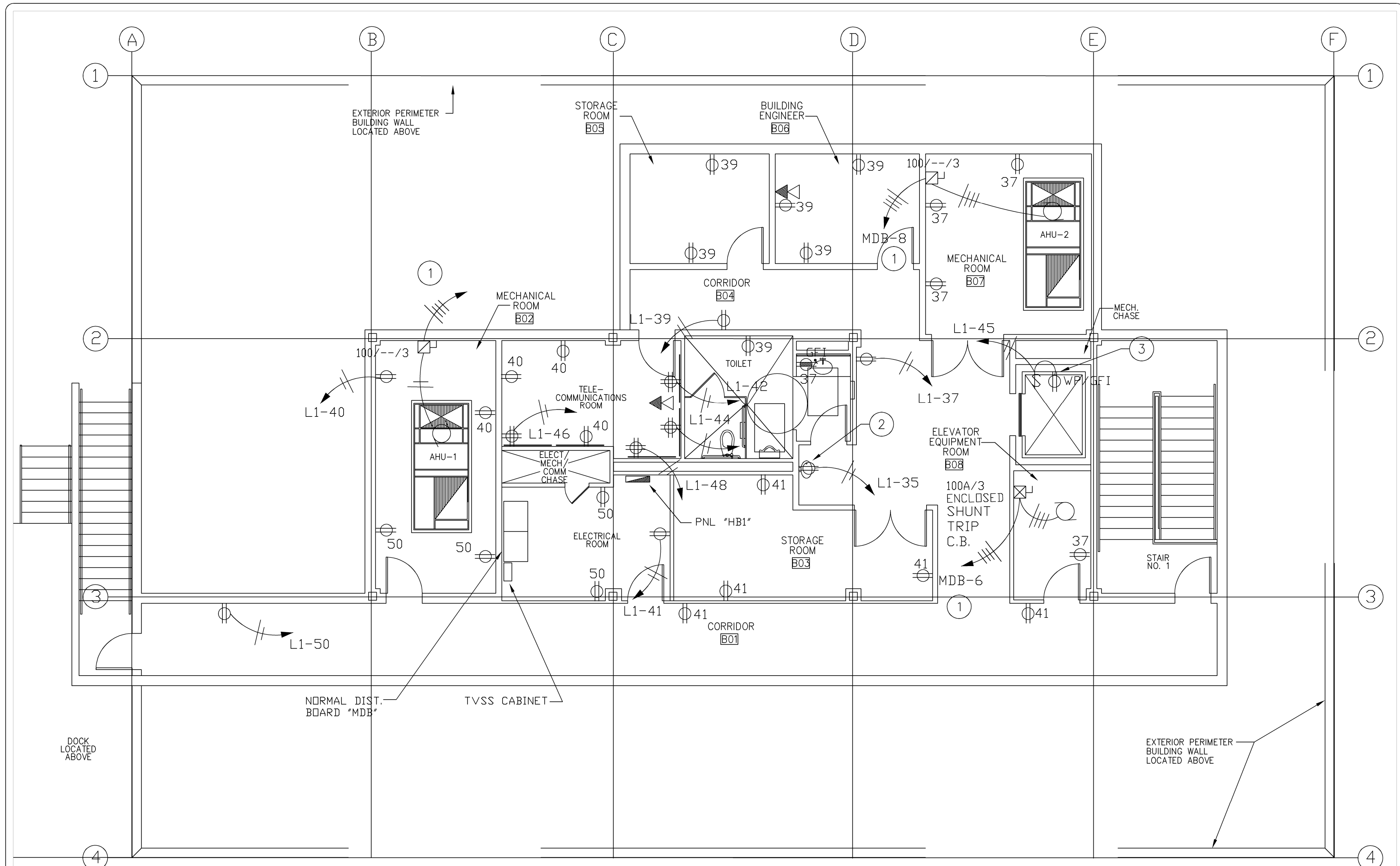
BASEMENT FLOOR PLAN - POWER SCALE: 3/16" = 1'-0"
