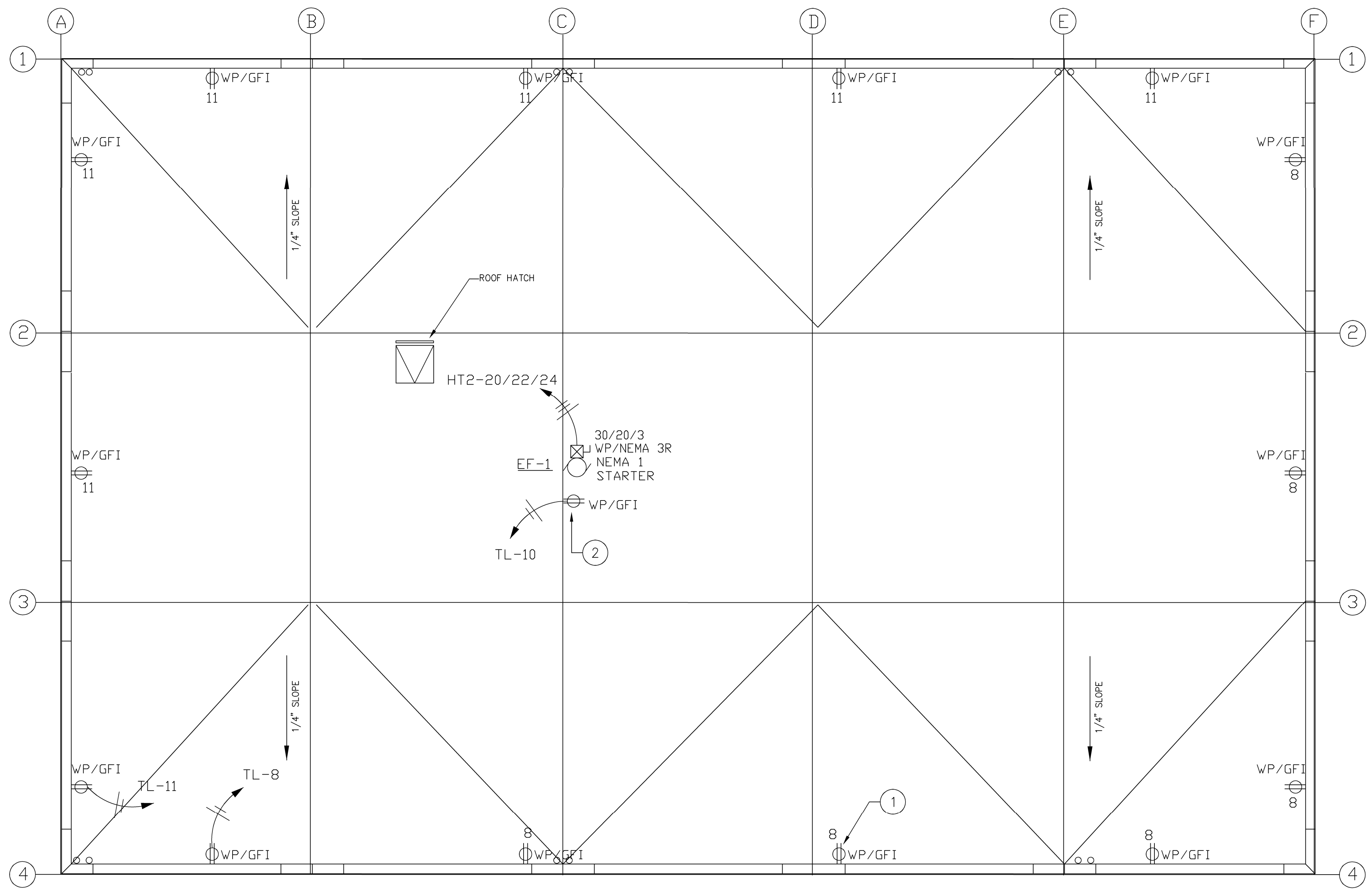
ROOF PLAN - POWER SCALE: 3/16" = 1'-0"
