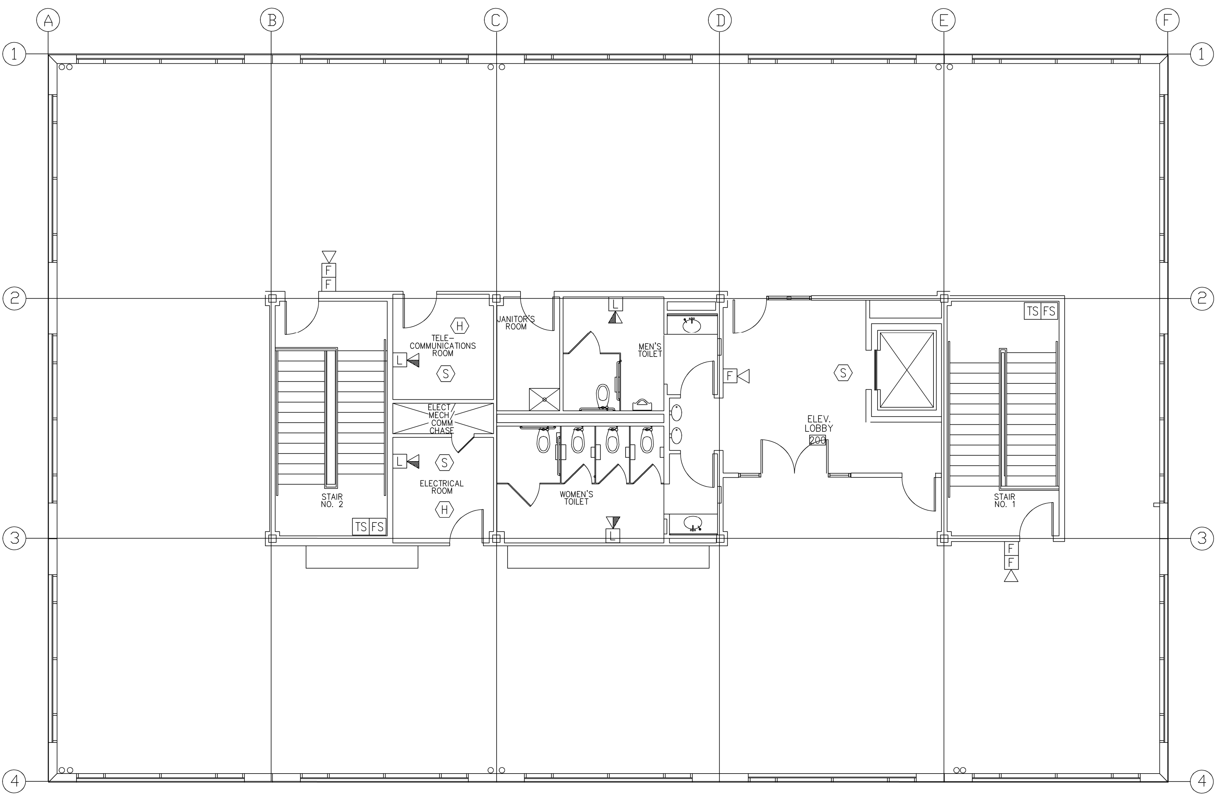
TYPICAL FLOOR ( 2ND TO 3RD) PLAN - FIRE ALARM SYSTEM
