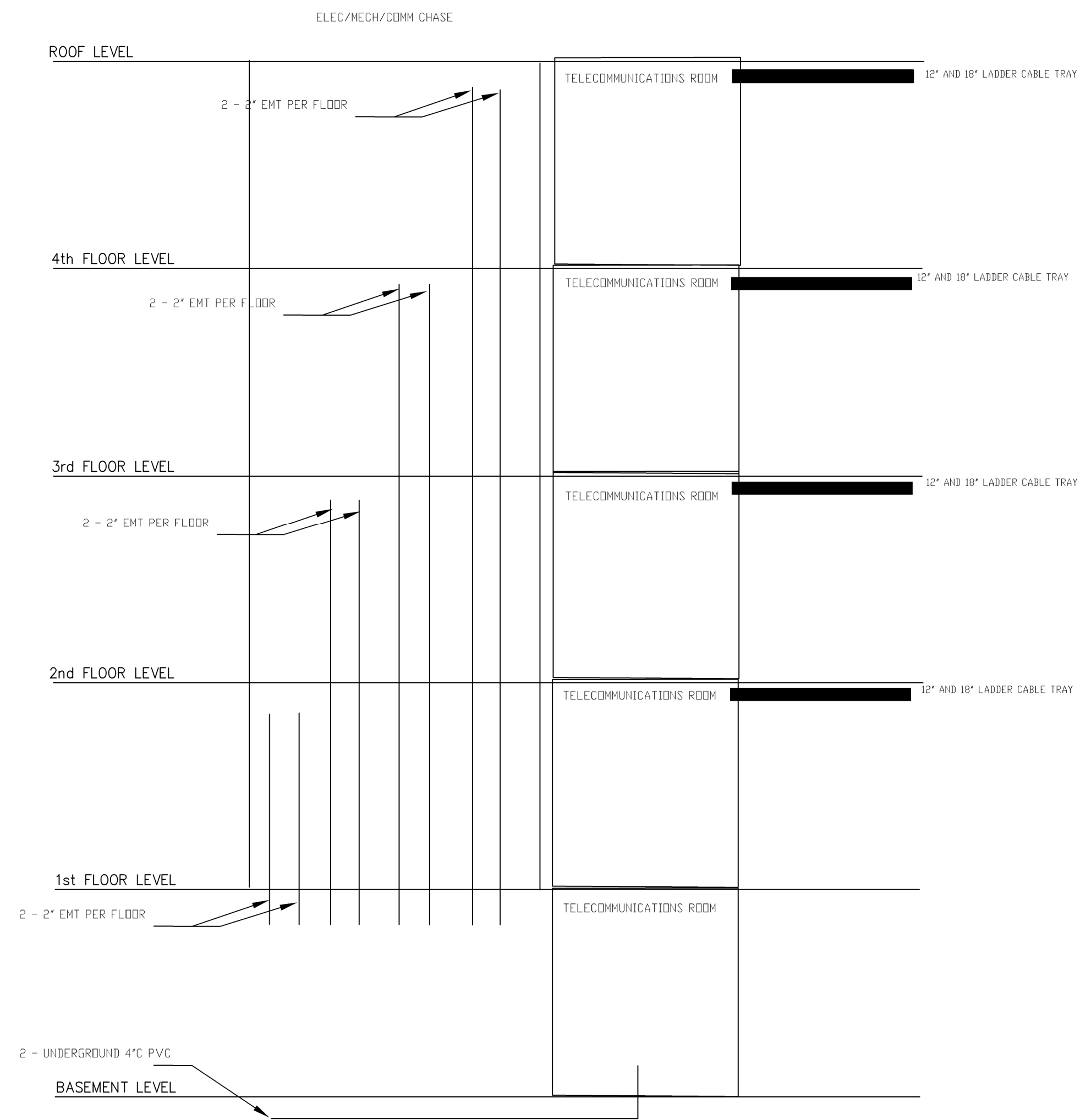
TELECOMMUNICATIONS RISER DIAGRAM NO SCALE
