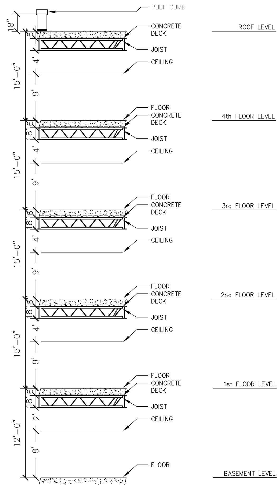
TYPICAL BUILDING SECTION NO SCALE
