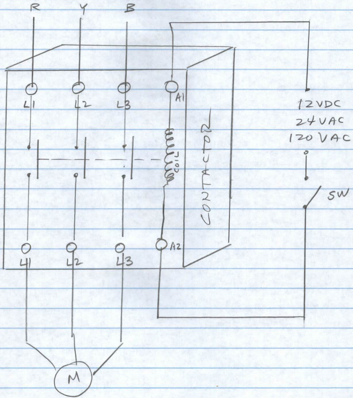
3-phase Contactor
