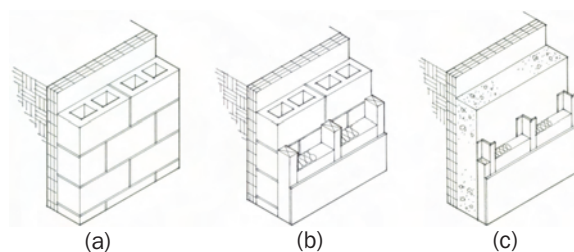
Figure 4-9. (EN10) Below grade walls—outer surface of the wall is in contact with the earth, and the inside surface is adjacent to conditioned or semi-heated space.
