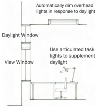
Figure 4-20. (EN38) Daylight window and view window.
