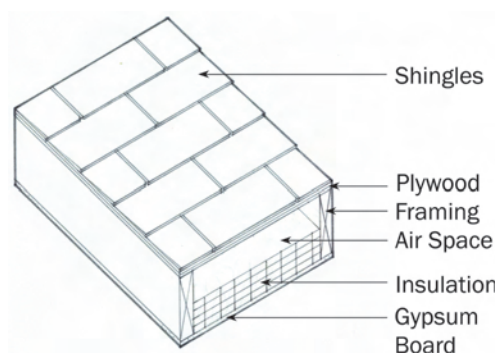
Figure 4-4. (EN5) Wood joists, single rafter.
