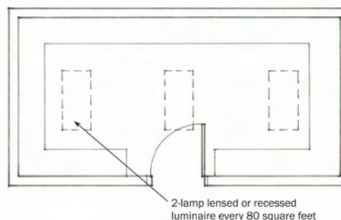
Figure 4-29. (EL16) Layout for storage area.
