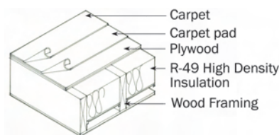
Figure 4-11. (EN12) Floors, wood frame.
