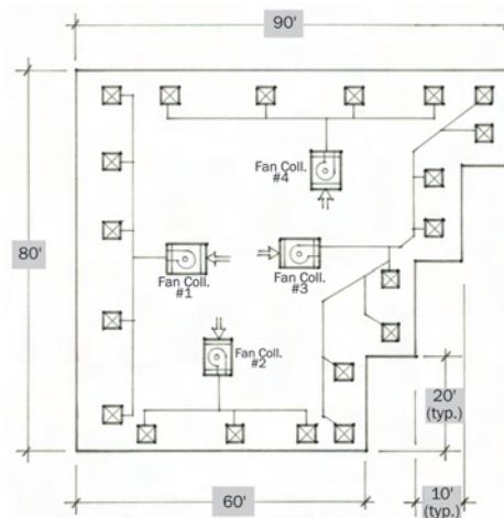
Figure 4-32. (HV13) Perimeter system zoning.
