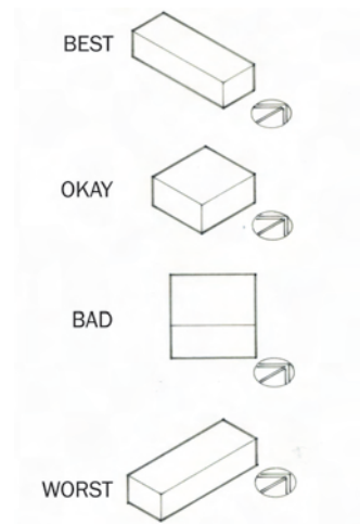
Elongate building in East/West orientation to maximize windows on North/South.
