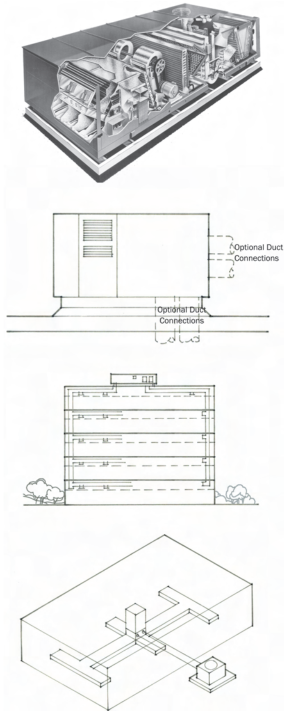
Figure 4-30. (HV1) Typical HVAC equipment and duct system layouts.
