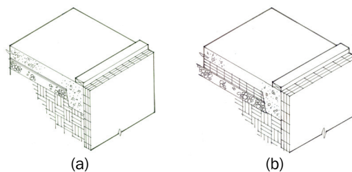
Figure 4-12. (EN13) Slab-on-grade floors, unheated. No heating elements either within or below the slab.
